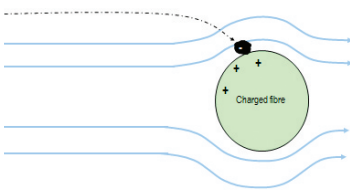
Figure 2d: Transport mechanisms in particle separation on fibres – Electrostatics
