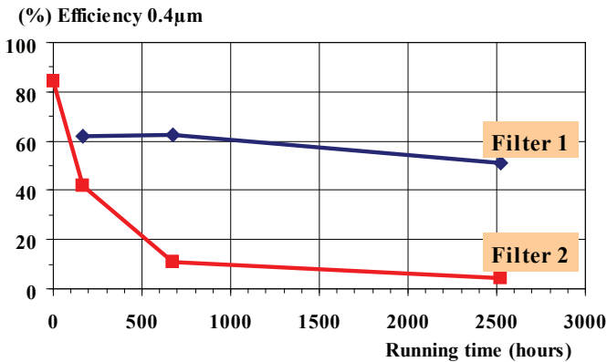
Figure 3: Increase of efficiency due to electrostatic charge
