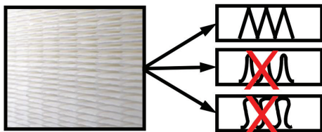
Figure 7: Correct and incorrect pleat shape configuration
