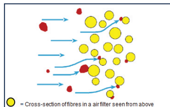
Figure 2a: Transport mechanisms in particle separation on fibres – Interception
