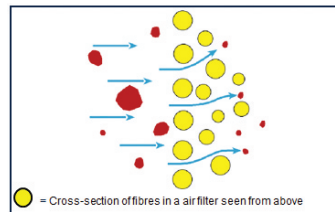
Figure 2b: Transport mechanisms in particle separation on fibres – Inertia effect
