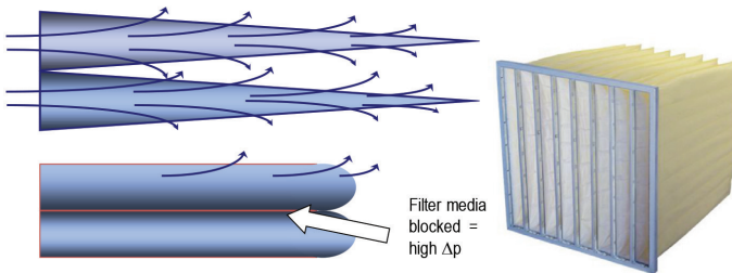
Figure 6: Schematic air flow in correctly designed and poor quality bag filter
