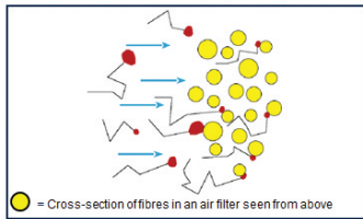
Figure 2c: Transport mechanisms in particle separation on fibres – Diffusion
