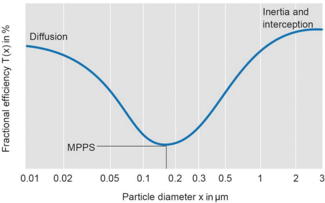
Figure 4: Transport mechanisms in particle separation on fibres
