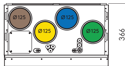
CASA R3 L Flat, left-hand version
